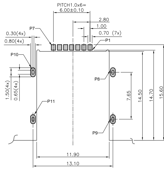
RERECOMMENDED P.C.BOARD LAYOUT
