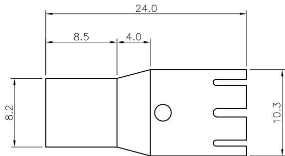
BACK SHELL
